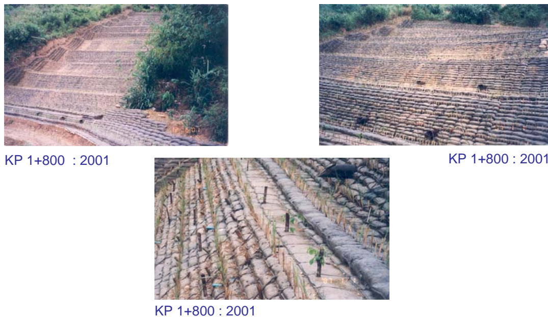
Figure 9 : KP 1+800, The application of jute sacks and vetiver grass were used for rebuilding laddered berms.
