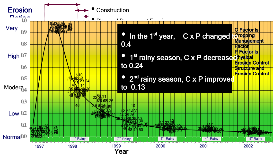
Figure 3 : Rehabilitation performance i.e. multiplication results of the C and P Factor for each KP.
