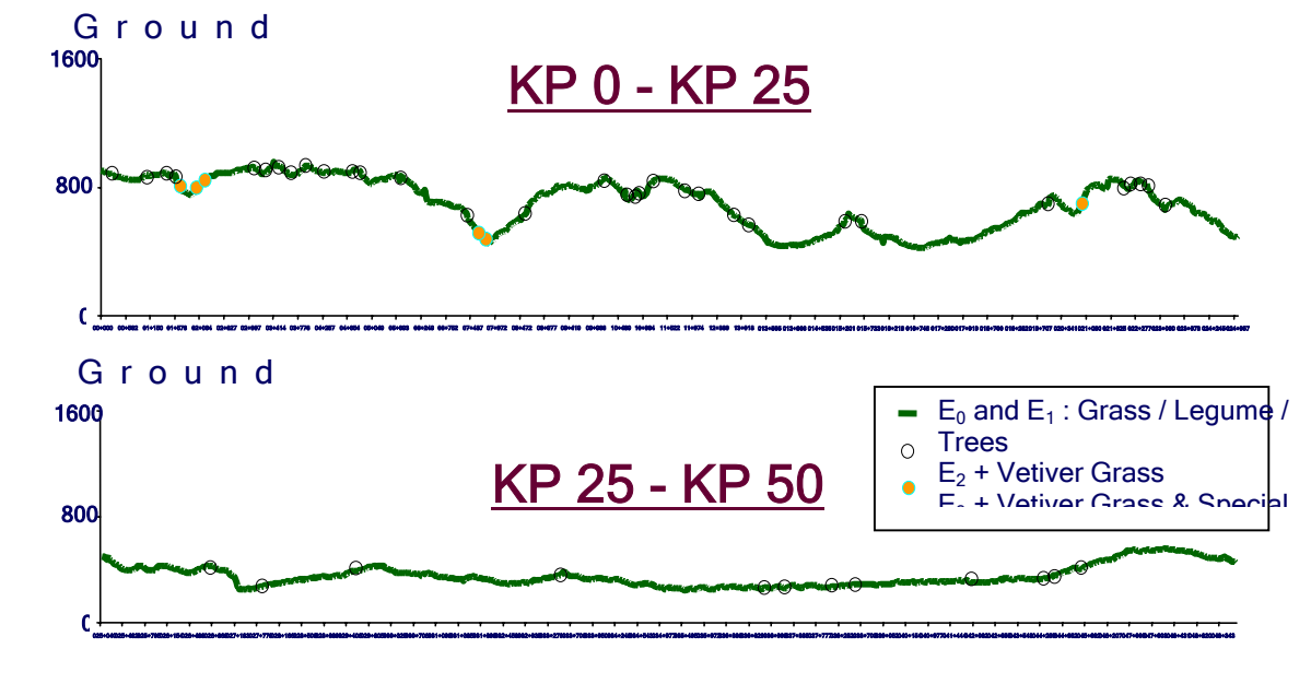
Figure 2 : The Erosion Rating Risk were identified to the construction profile
