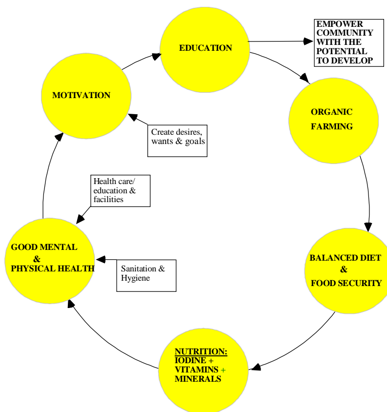
Fig. 2 Goals Diagram
