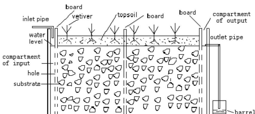
Figure 1. A cross-section view of the subsurface flow wetland
